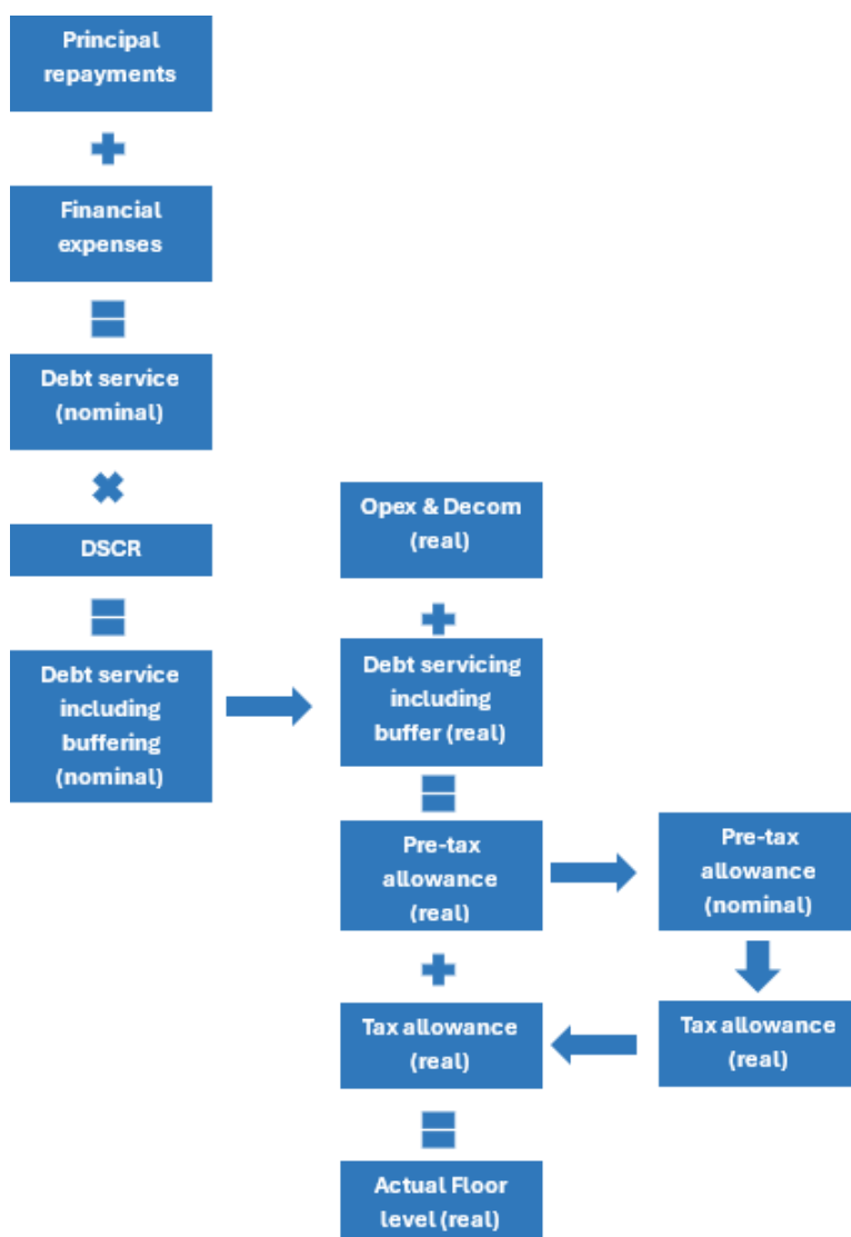
Figure 2: Building blocks of the LDES CFFM ACOD floor level
